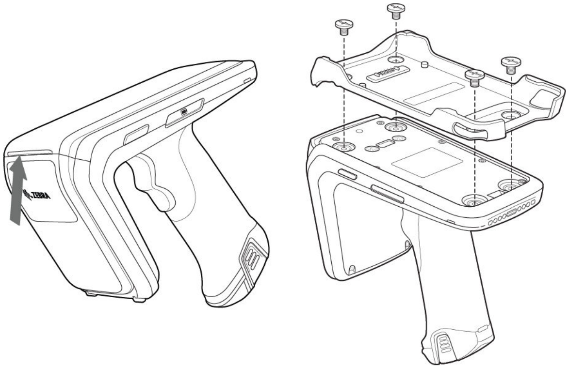
Figure 2 Adapter Installation
